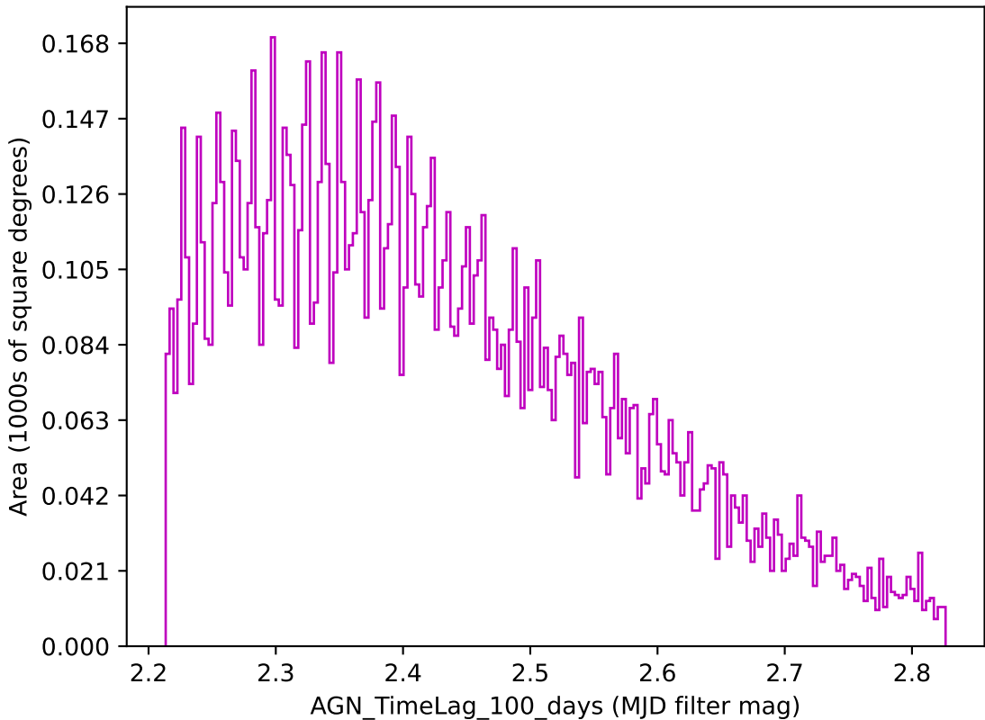
too_elab_r16_d3_gz_v3.4_10yrs z band: AGN_TimeLag_100_days
