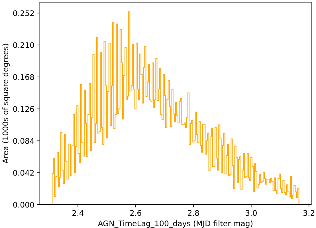
too_elab_r16_d3_gz_v3.4_10yrs r band: AGN_TimeLag_100_days
