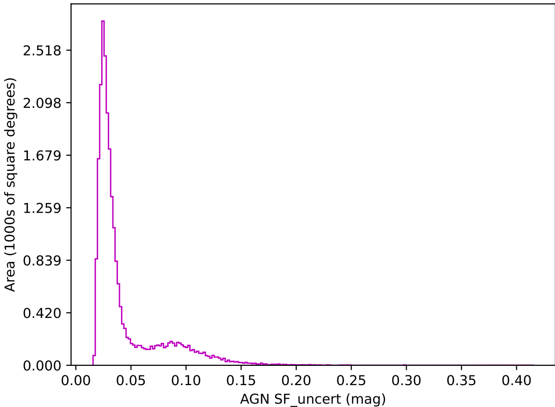
too_elab_r16_d3_gz_v3.4_10yrs z band: AGN SF_uncert
