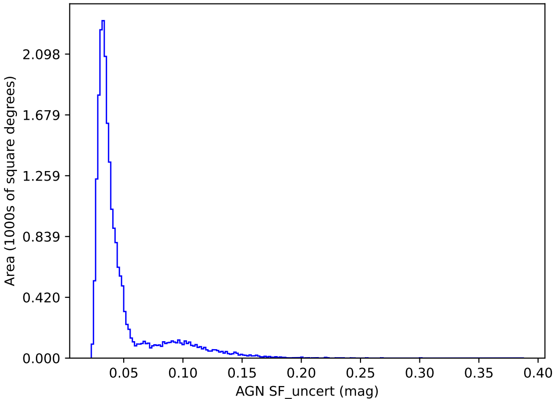
too_elab_r16_d3_gz_v3.4_10yrs y band: AGN SF_uncert
