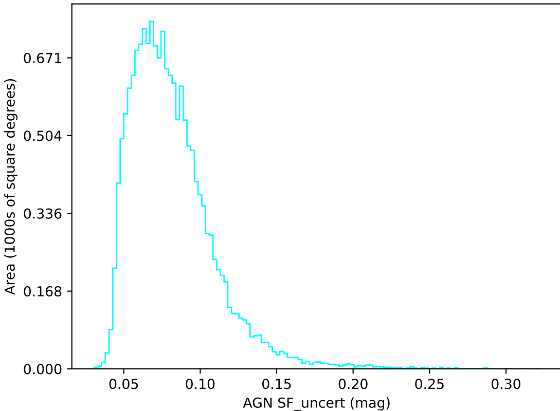
too_elab_r16_d3_gz_v3.4_10yrs u band: AGN SF_uncert
