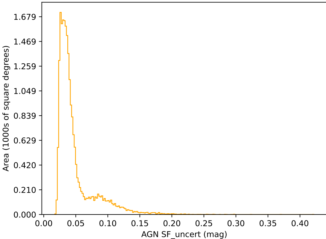
too_elab_r16_d3_gz_v3.4_10yrs r band: AGN SF_uncert
