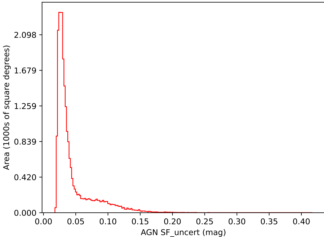
too_elab_r16_d3_gz_v3.4_10yrs i band: AGN SF_uncert
