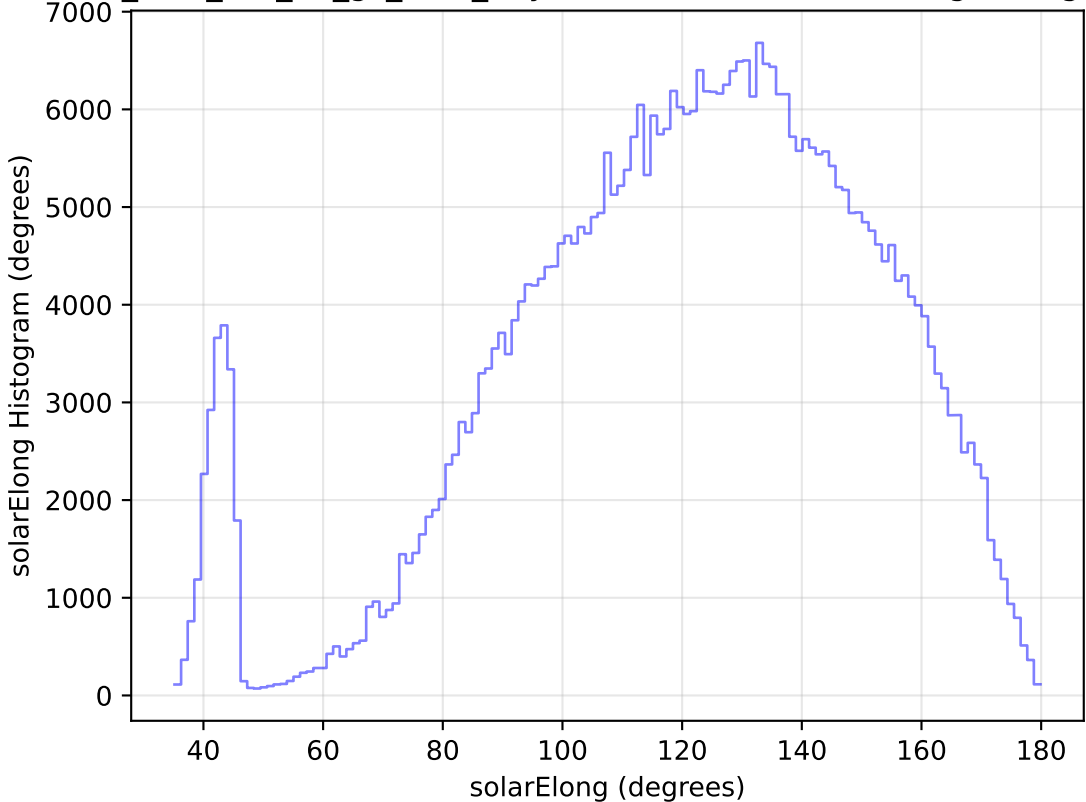
too_elab_r16_d3_gz_v3.4_10yrs WFD z band: solarElong Histogram
