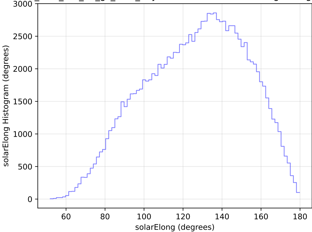
too_elab_r16_d3_gz_v3.4_10yrs WFD u band: solarElong Histogram
