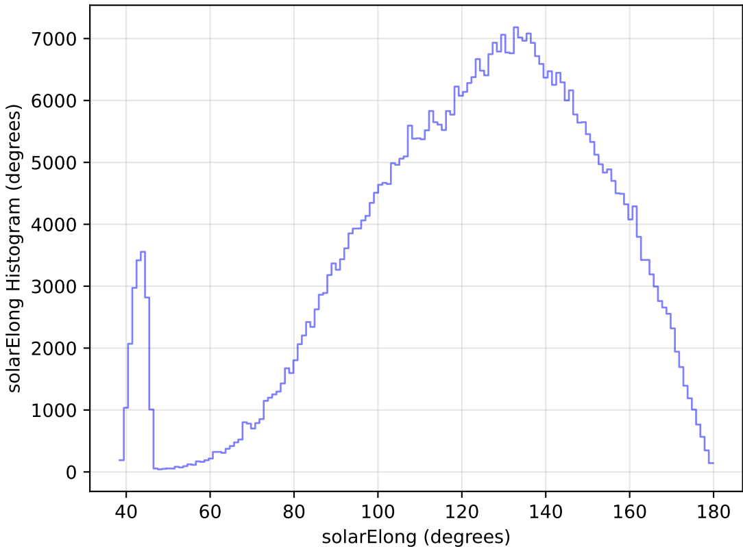
too_elab_r16_d3_gz_v3.4_10yrs WFD r band: solarElong Histogram
