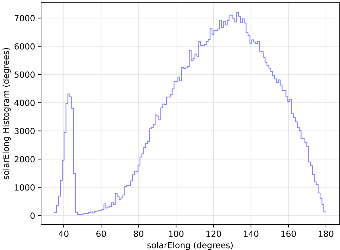
too_elab_r16_d3_gz_v3.4_10yrs WFD i band: solarElong Histogram
