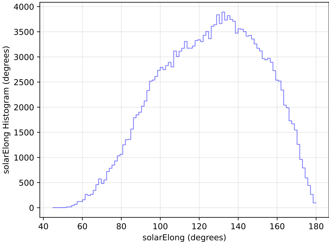
too_elab_r16_d3_gz_v3.4_10yrs WFD g band: solarElong Histogram
