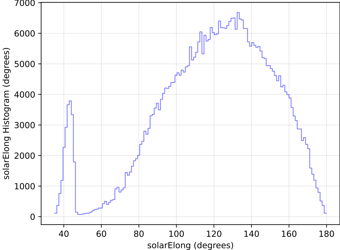
too_elab_r16_d3_gz_v3.4_10yrs All sky z band: solarElong Histogram
