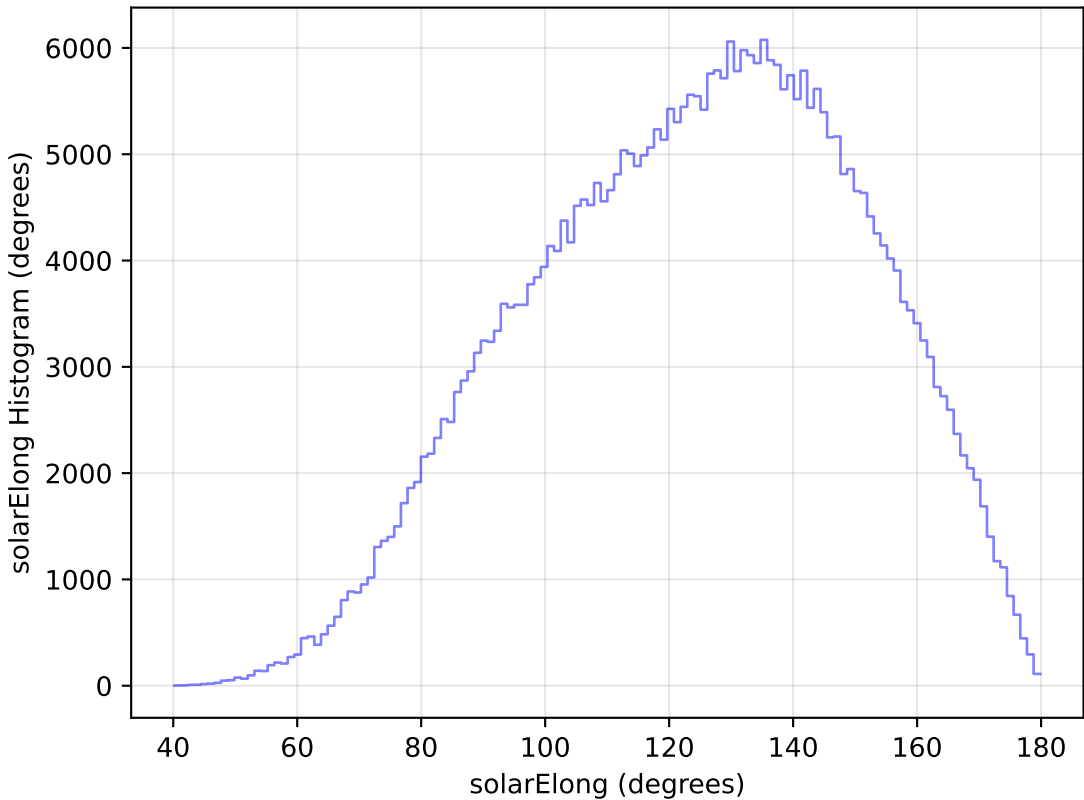
too_elab_r16_d3_gz_v3.4_10yrs All sky y band: solarElong Histogram
