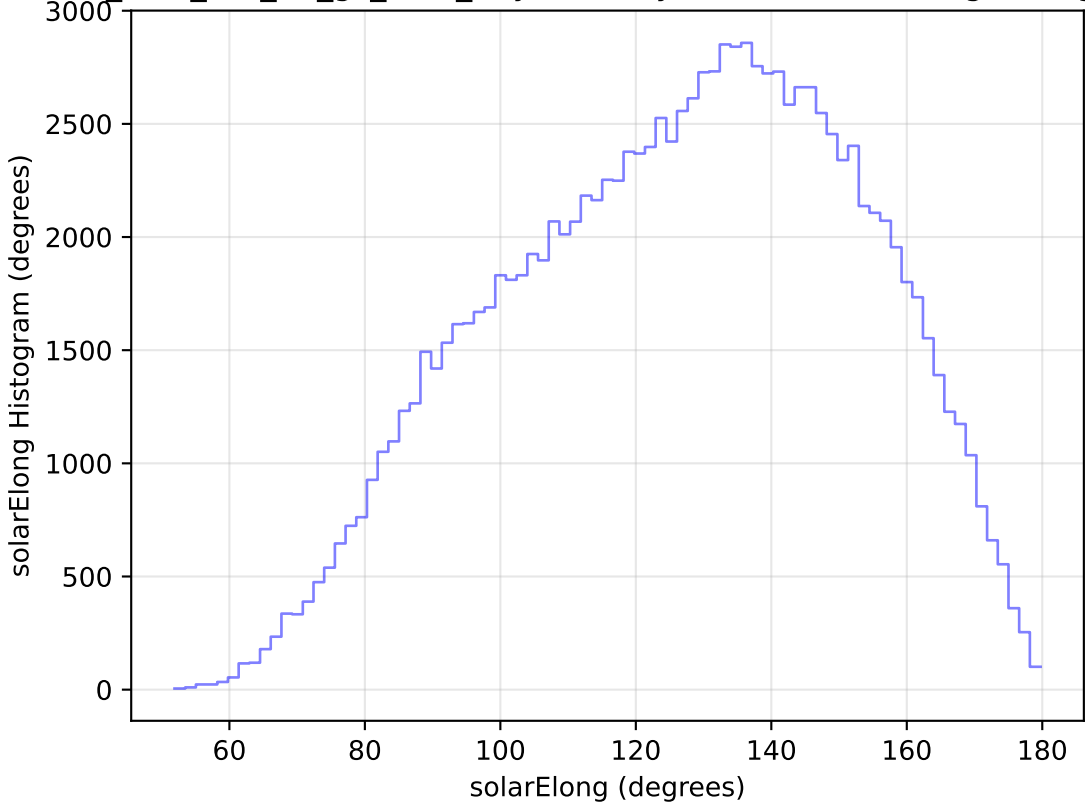
too_elab_r16_d3_gz_v3.4_10yrs All sky u band: solarElong Histogram
