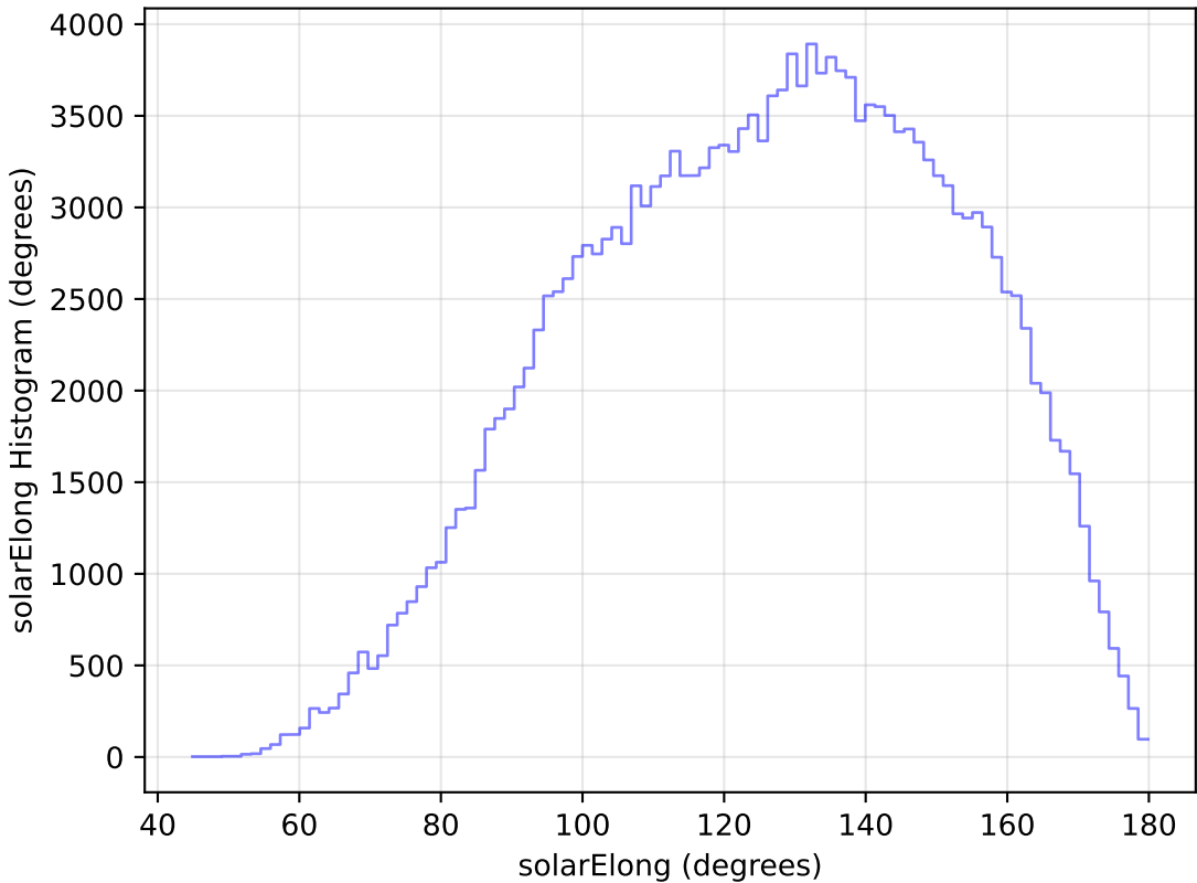
too_elab_r16_d3_gz_v3.4_10yrs All sky g band: solarElong Histogram
