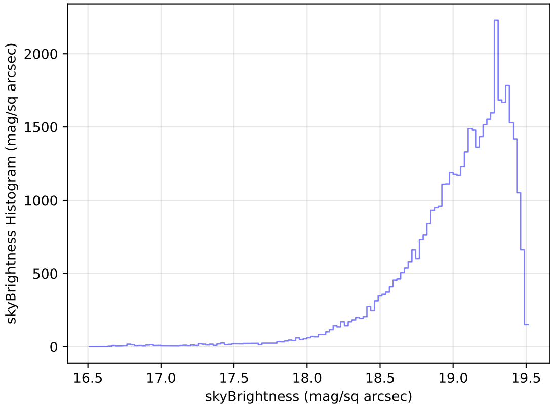
too_elab_r16_d3_gz_v3.4_10yrs Yr 1 z band: skyBrightness Histogram
