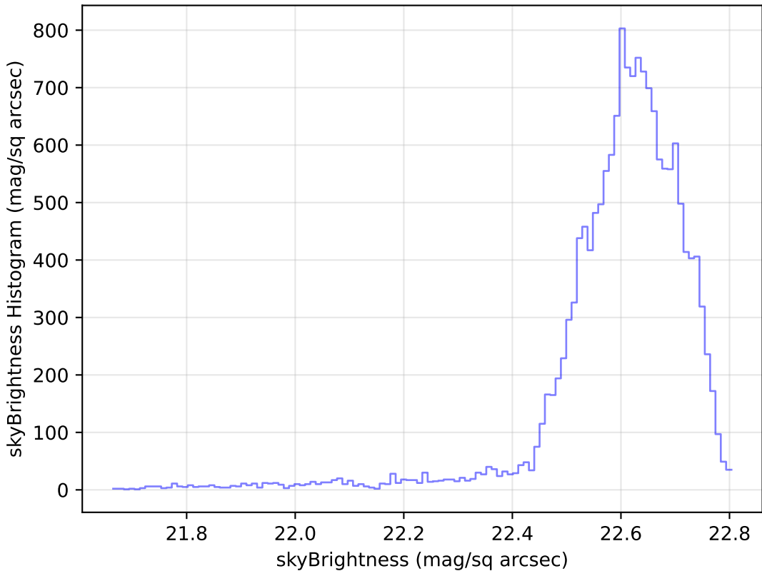
too_elab_r16_d3_gz_v3.4_10yrs Yr 1 u band: skyBrightness Histogram
