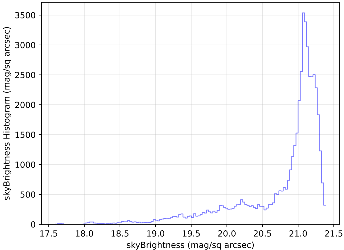
too_elab_r16_d3_gz_v3.4_10yrs Yr 1 r band: skyBrightness Histogram
