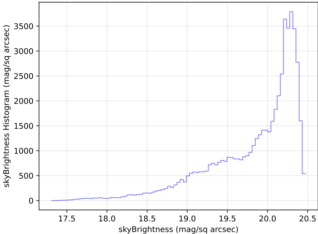
too_elab_r16_d3_gz_v3.4_10yrs Yr 1 i band: skyBrightness Histogram
