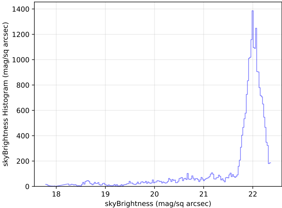
too_elab_r16_d3_gz_v3.4_10yrs Yr 1 g band: skyBrightness Histogram
