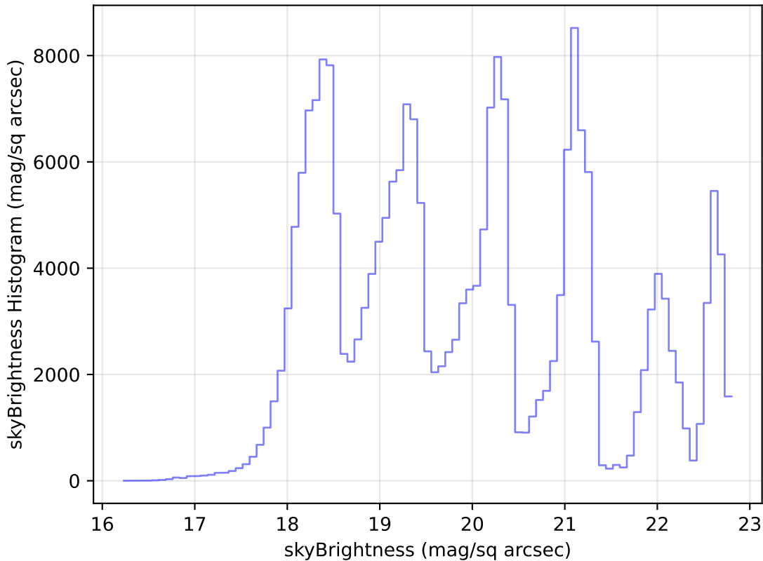
too_elab_r16_d3_gz_v3.4_10yrs Yr 1 all bands: skyBrightness Histogram
