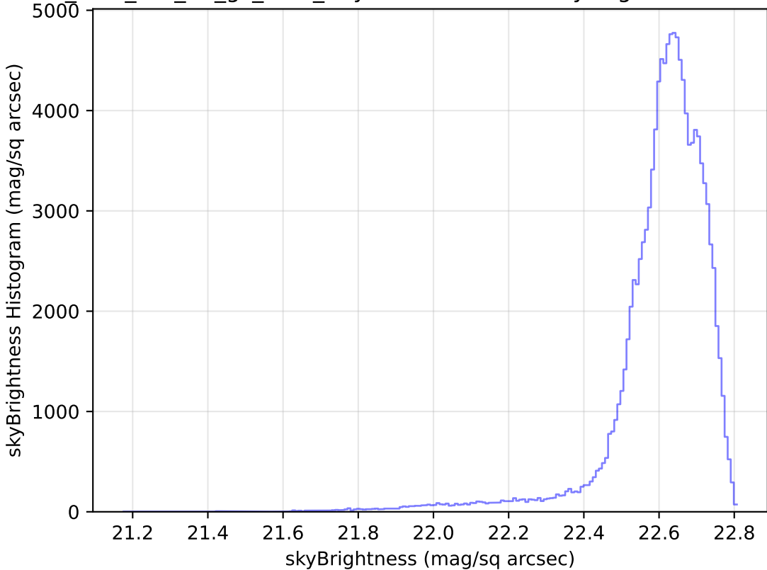
too_elab_r16_d3_gz_v3.4_10yrs WFD u band: skyBrightness Histogram
