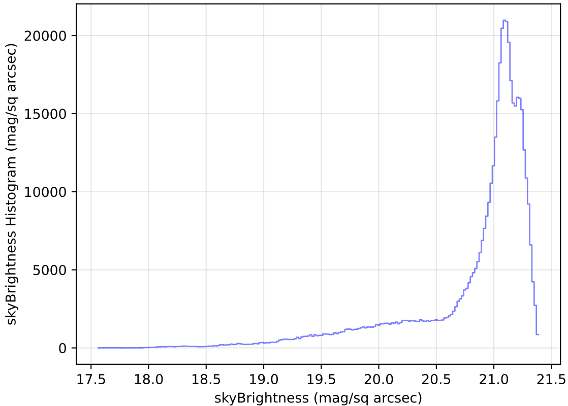
too_elab_r16_d3_gz_v3.4_10yrs WFD r band: skyBrightness Histogram
