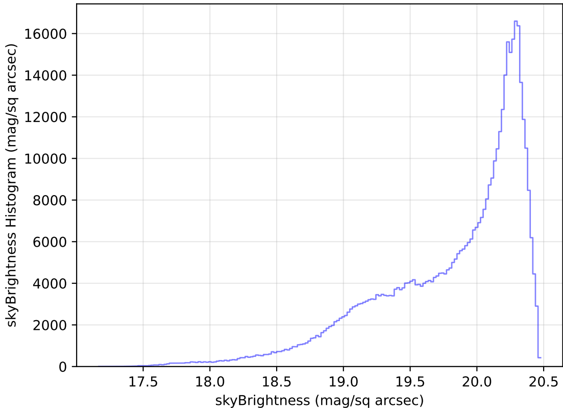
too_elab_r16_d3_gz_v3.4_10yrs WFD i band: skyBrightness Histogram
