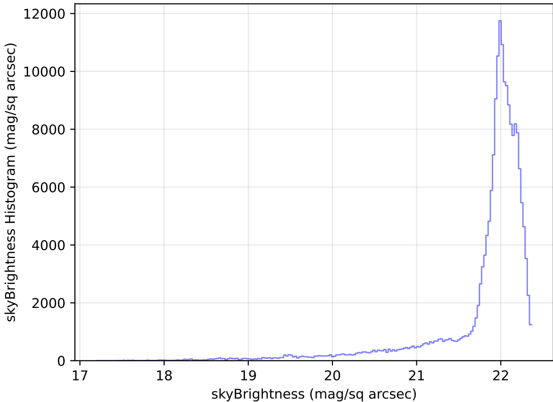
too_elab_r16_d3_gz_v3.4_10yrs WFD g band: skyBrightness Histogram
