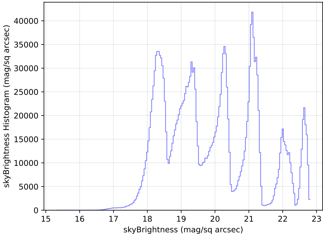
too_elab_r16_d3_gz_v3.4_10yrs WFD all bands: skyBrightness Histogram
