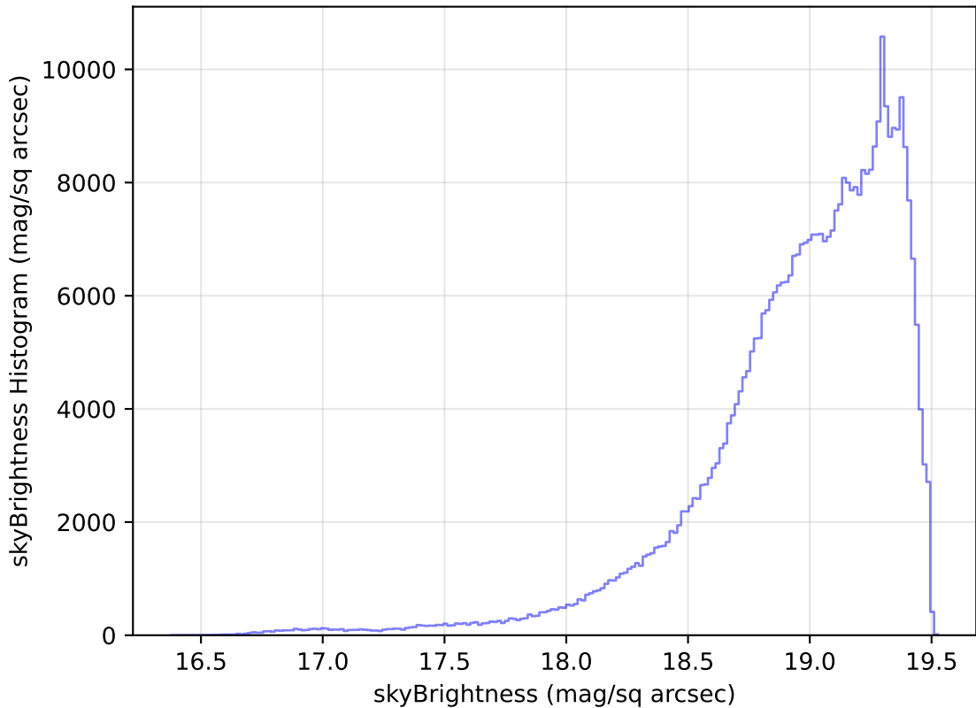
too_elab_r16_d3_gz_v3.4_10yrs All sky z band: skyBrightness Histogram
