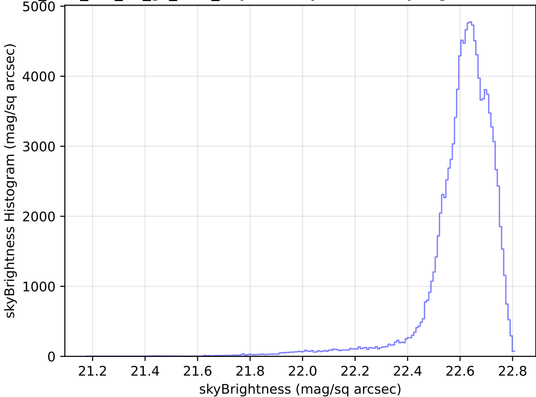
too_elab_r16_d3_gz_v3.4_10yrs All sky u band: skyBrightness Histogram
