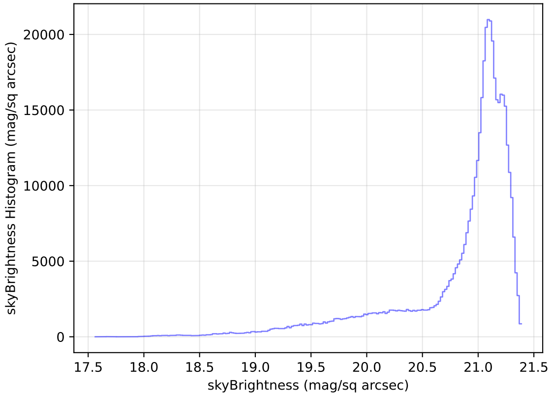
too_elab_r16_d3_gz_v3.4_10yrs All sky r band: skyBrightness Histogram
