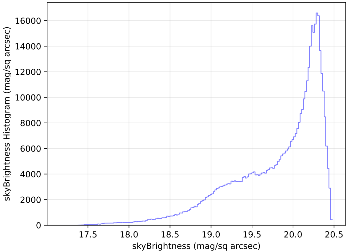
too_elab_r16_d3_gz_v3.4_10yrs All sky i band: skyBrightness Histogram
