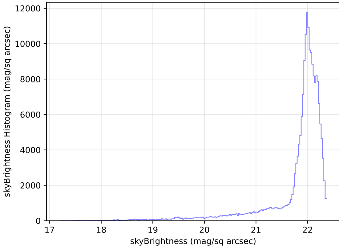
too_elab_r16_d3_gz_v3.4_10yrs All sky g band: skyBrightness Histogram
