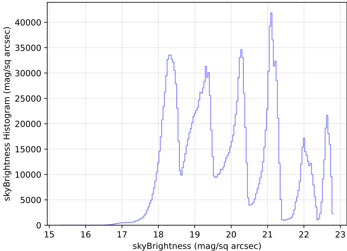
too_elab_r16_d3_gz_v3.4_10yrs All sky all bands: skyBrightness Histogram
