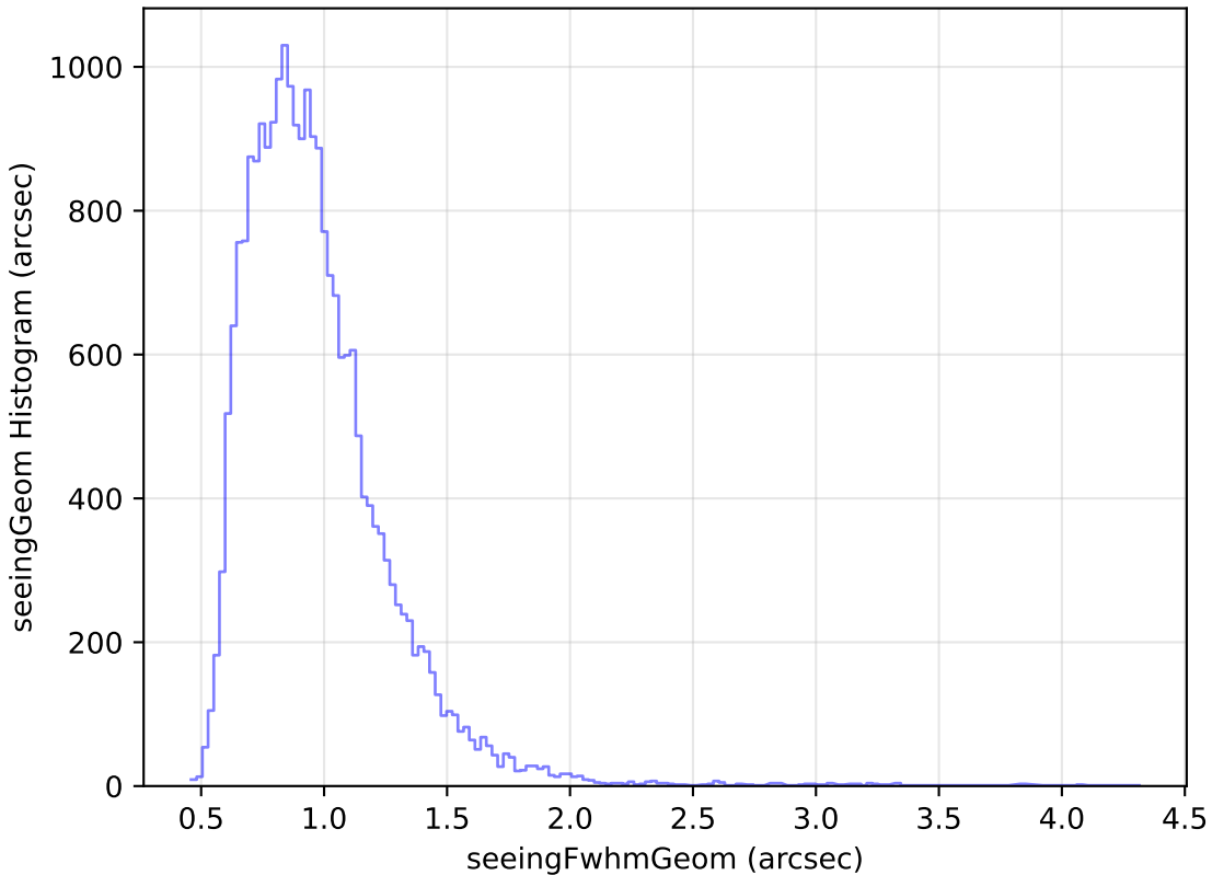
too_elab_r16_d3_gz_v3.4_10yrs Yr 1 g band: seeingGeom Histogram
