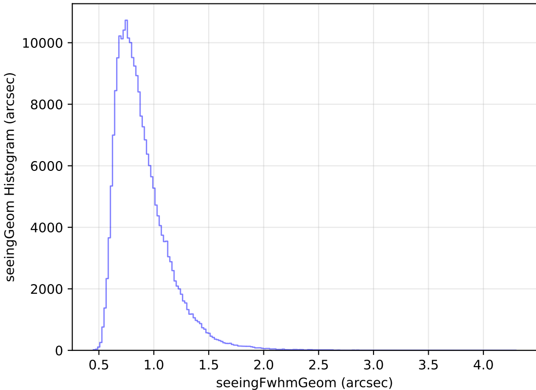
too_elab_r16_d3_gz_v3.4_10yrs Yr 1 all bands: seeingGeom Histogram
