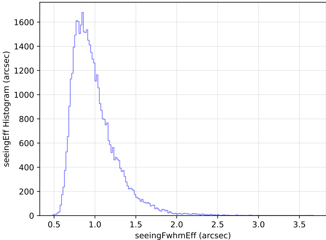
too_elab_r16_d3_gz_v3.4_10yrs Yr 1 z band: seeingEff Histogram
