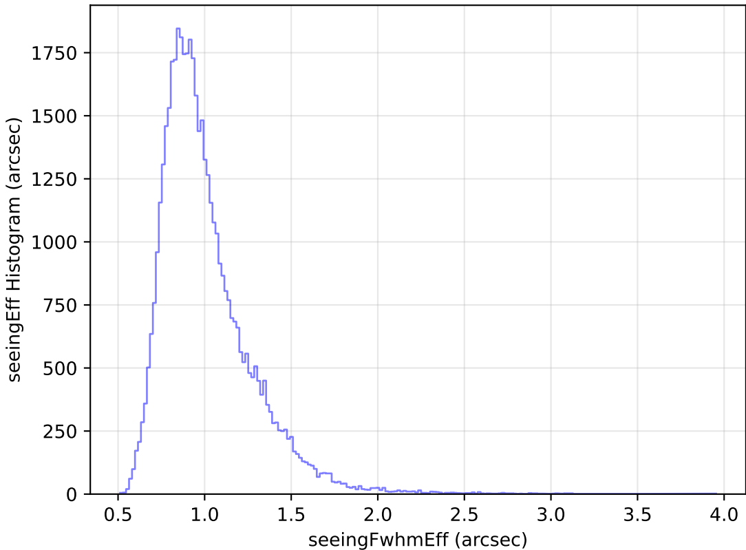
too_elab_r16_d3_gz_v3.4_10yrs Yr 1 y band: seeingEff Histogram
