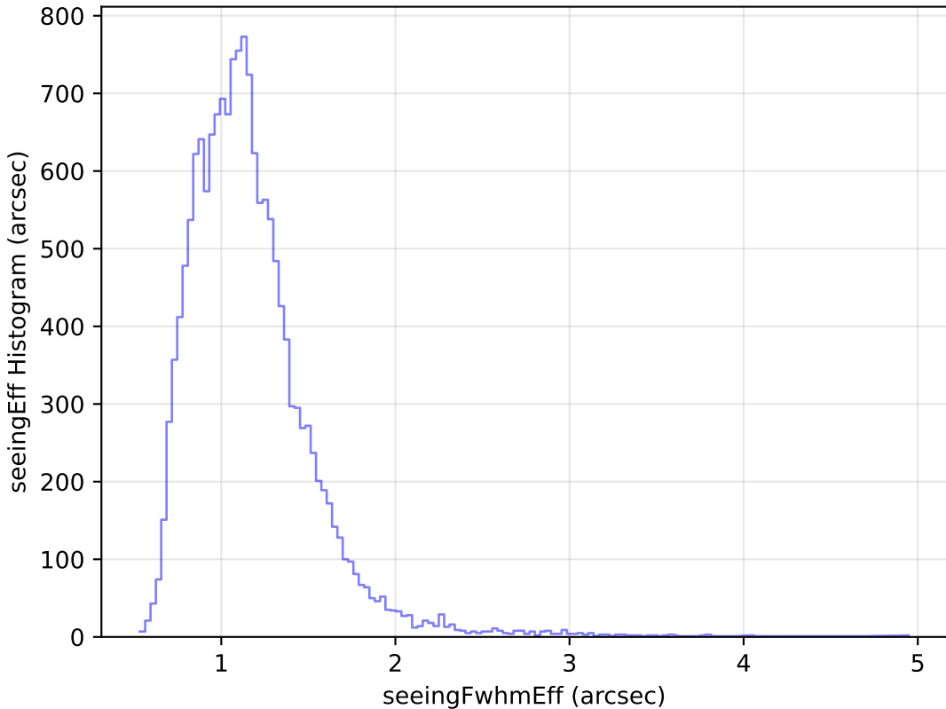
too_elab_r16_d3_gz_v3.4_10yrs Yr 1 u band: seeingEff Histogram
