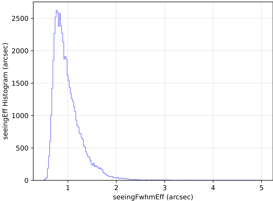
too_elab_r16_d3_gz_v3.4_10yrs Yr 1 i band: seeingEff Histogram
