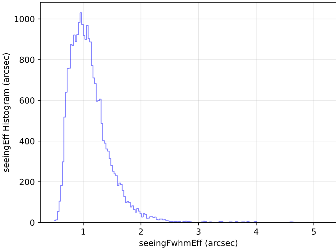
too_elab_r16_d3_gz_v3.4_10yrs Yr 1 g band: seeingEff Histogram
