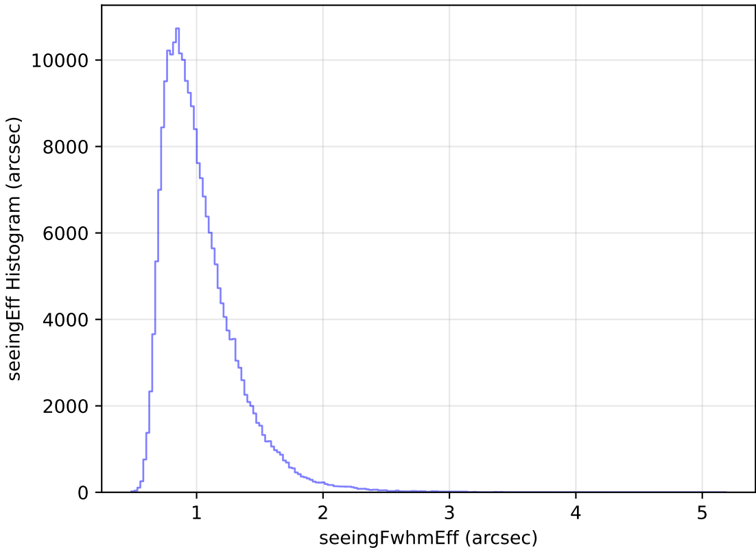
too_elab_r16_d3_gz_v3.4_10yrs Yr 1 all bands: seeingEff Histogram
