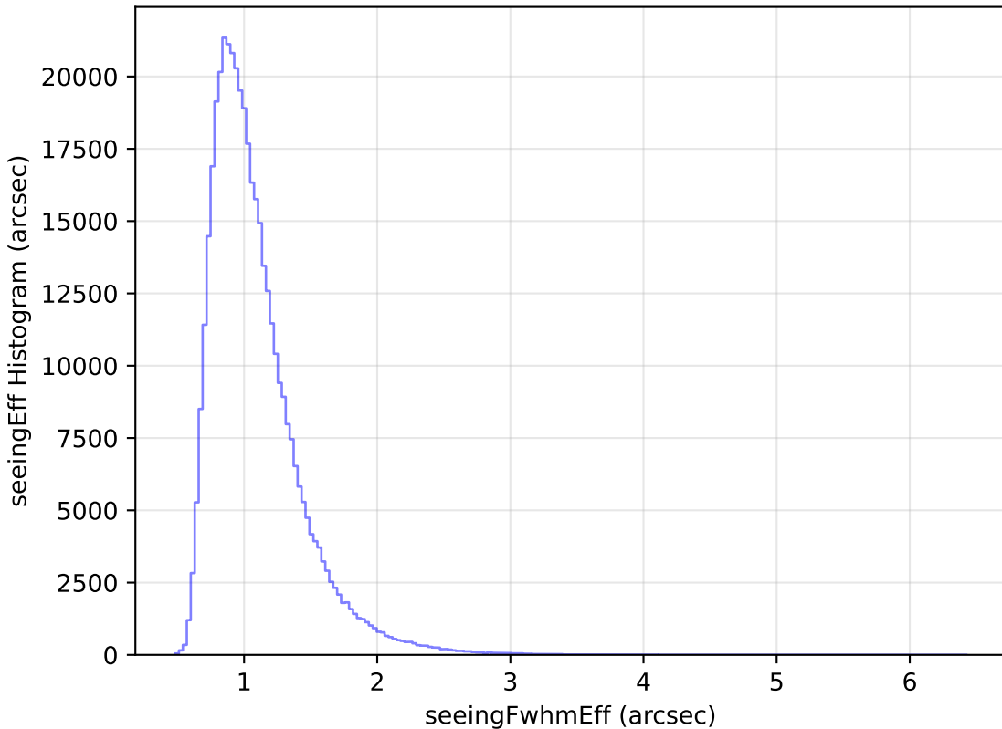
too_elab_r16_d3_gz_v3.4_10yrs WFD z band: seeingEff Histogram
