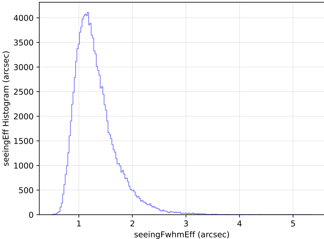
too_elab_r16_d3_gz_v3.4_10yrs WFD u band: seeingEff Histogram
