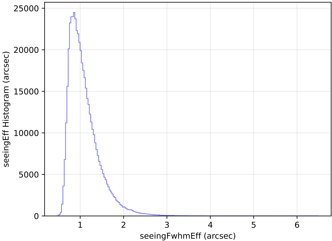
too_elab_r16_d3_gz_v3.4_10yrs WFD i band: seeingEff Histogram
