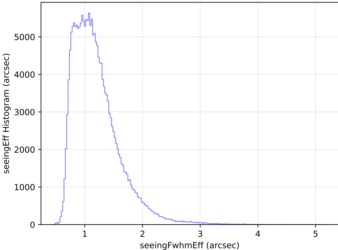
too_elab_r16_d3_gz_v3.4_10yrs WFD g band: seeingEff Histogram
