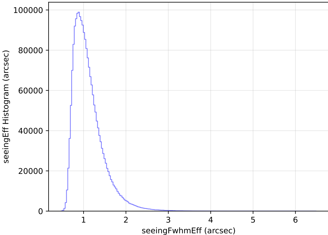
too_elab_r16_d3_gz_v3.4_10yrs WFD all bands: seeingEff Histogram
