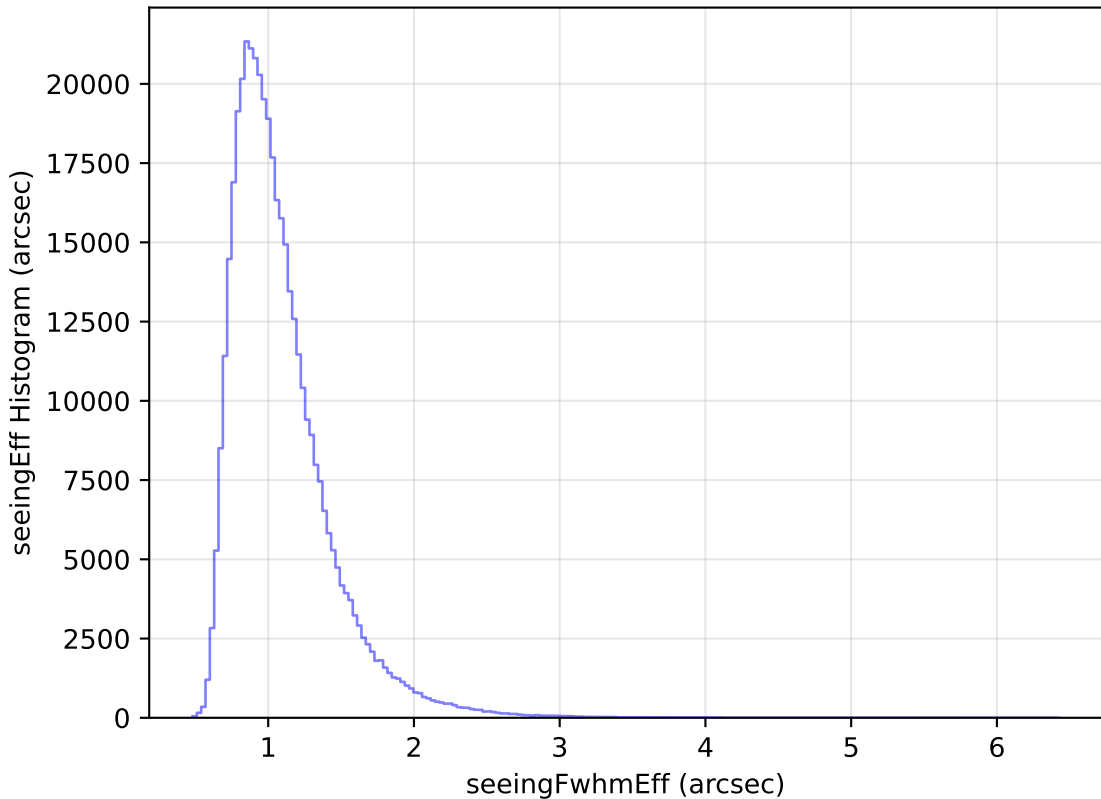
too_elab_r16_d3_gz_v3.4_10yrs All sky z band: seeingEff Histogram
