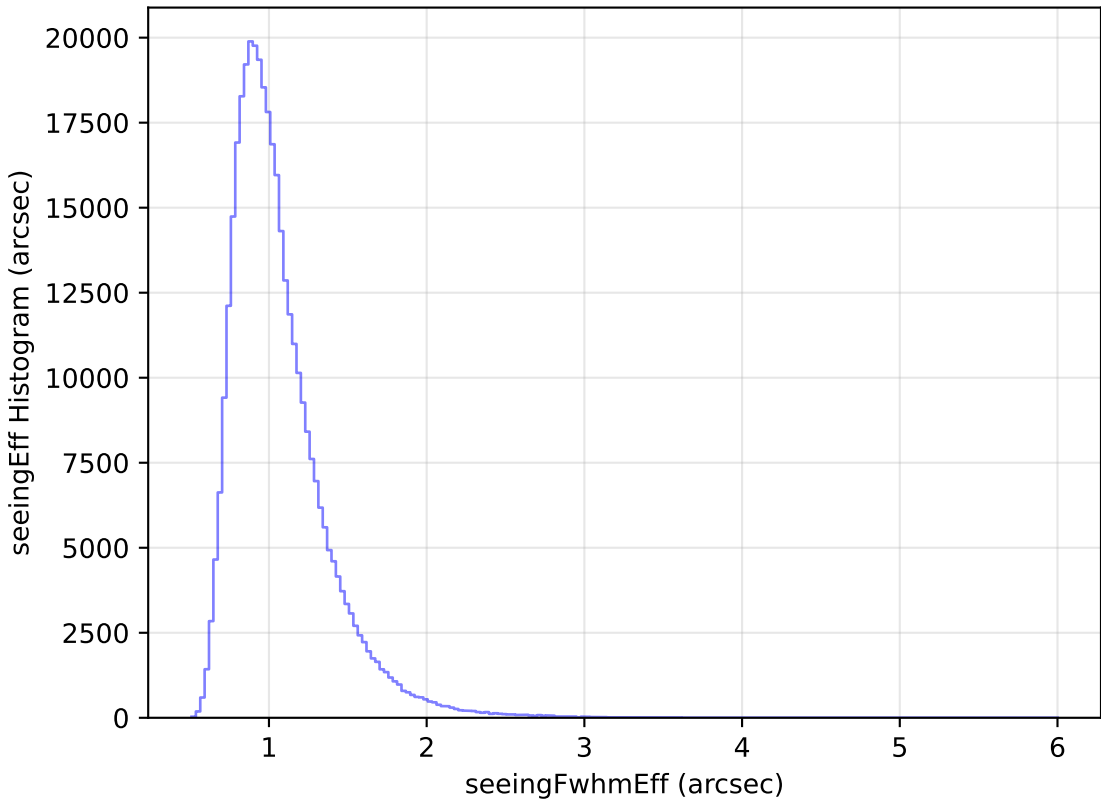
too_elab_r16_d3_gz_v3.4_10yrs All sky y band: seeingEff Histogram
