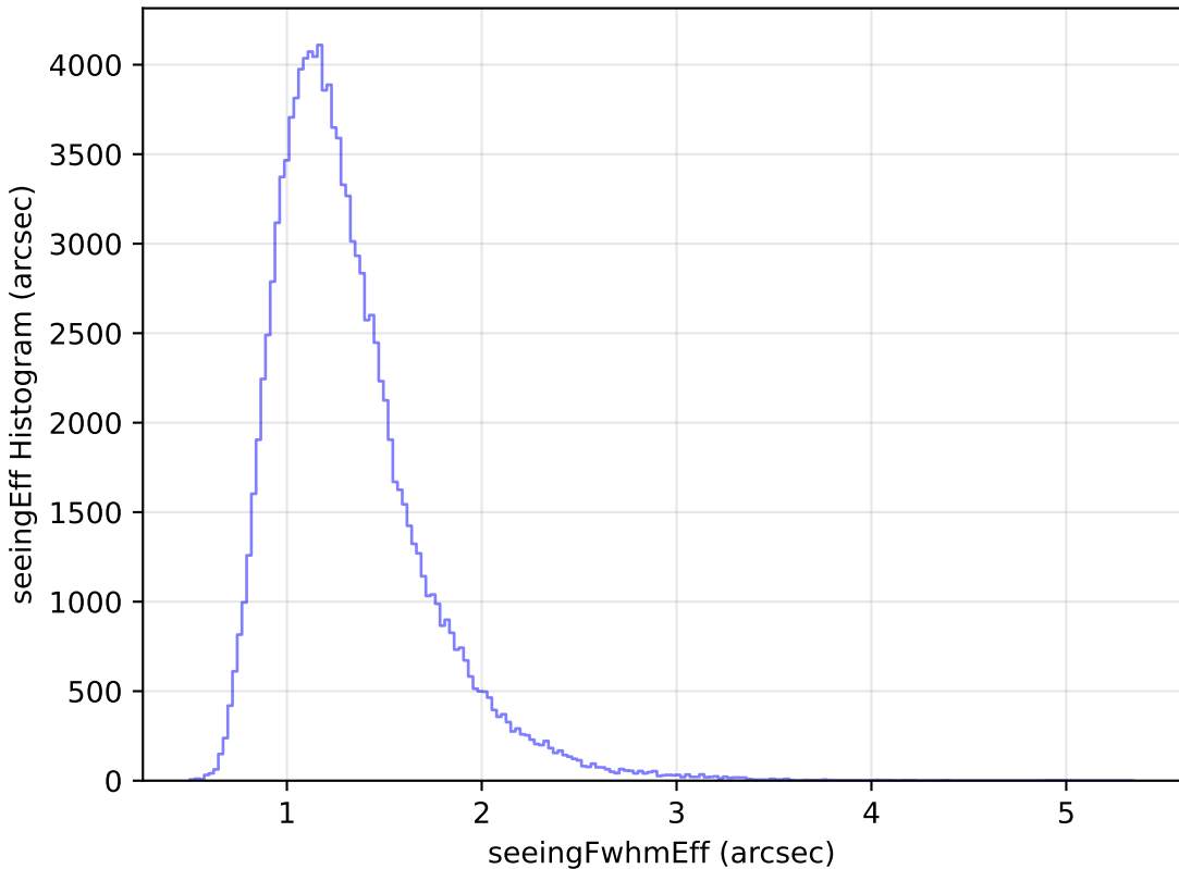
too_elab_r16_d3_gz_v3.4_10yrs All sky u band: seeingEff Histogram
