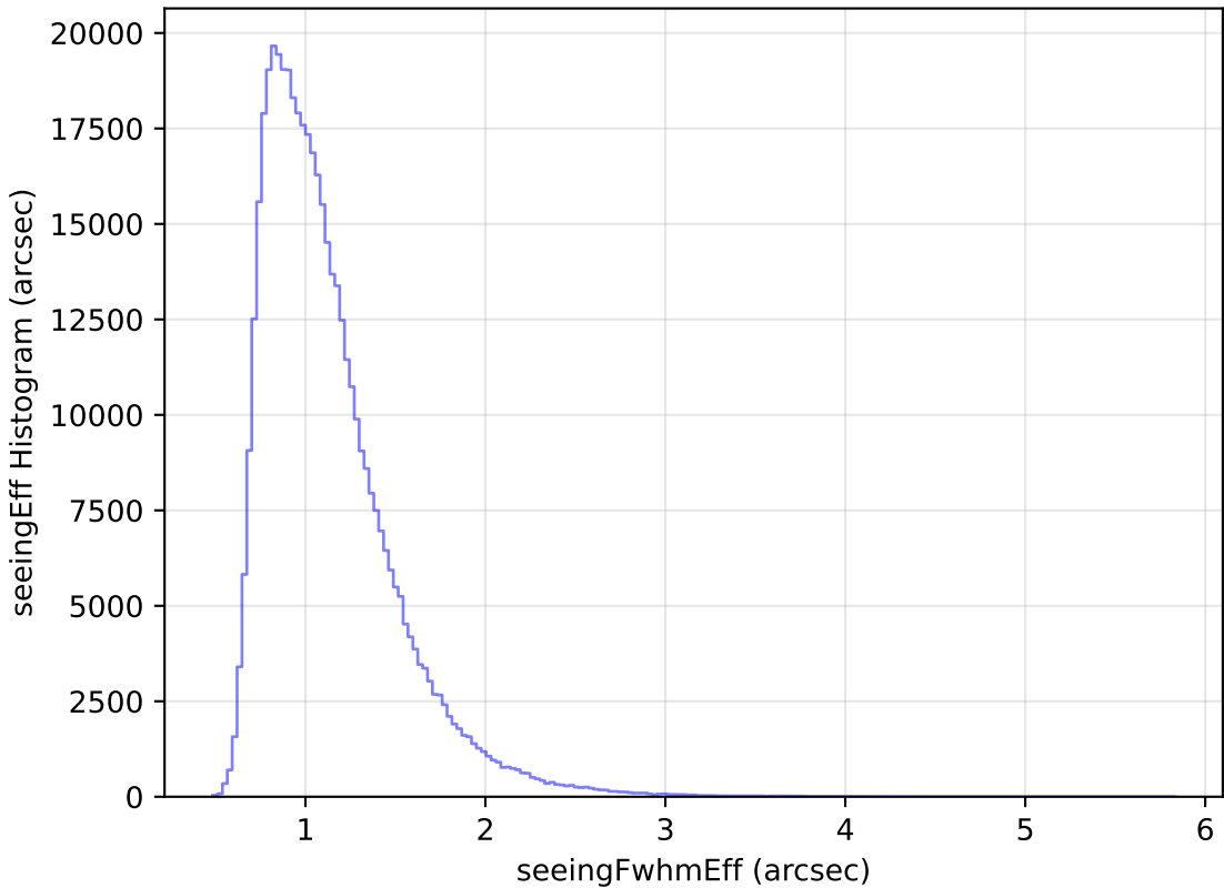
too_elab_r16_d3_gz_v3.4_10yrs All sky r band: seeingEff Histogram
